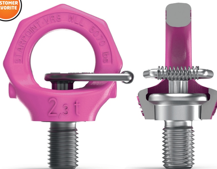
VRS-F (with Star profile key)
