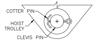
Diagram 5E. Installing cotter pin through trolley saddle clevis pin.
