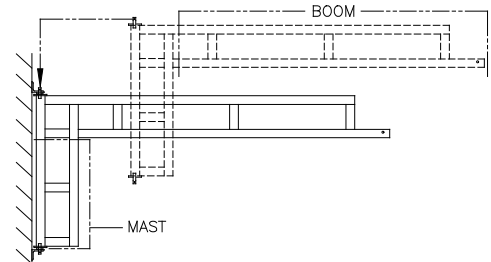
Diagram 2C. Installing boom weldment.
