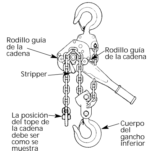
Figure 11. 6 Tonelada
