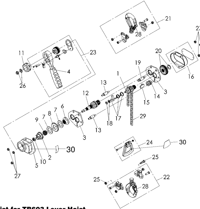
Figure 6 - TB603 Lever Hoist Exploded View
