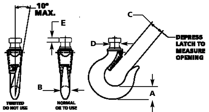
Figure 3 - Hook Inspection
